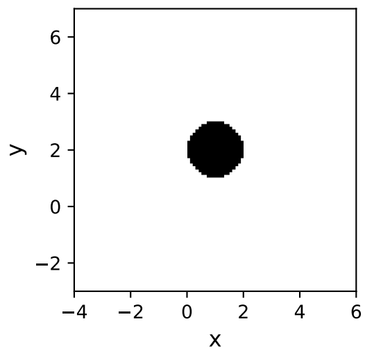
Disk2D
