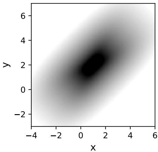
GeneralSersic2D, c=1.0
