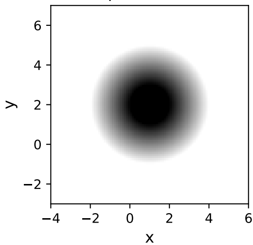
TrapezoidDisk2D
