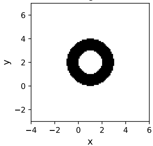
Ring2D
