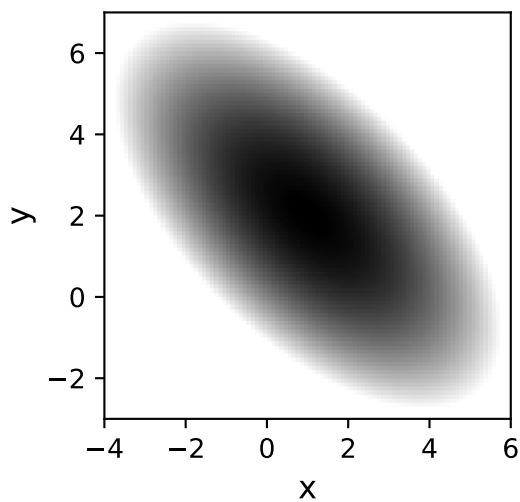
Gaussian2D
