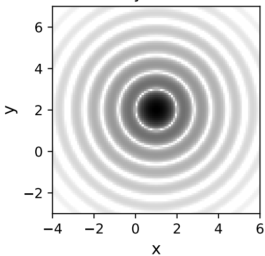
AiryDisk2D
