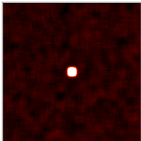
Box2DKernel
