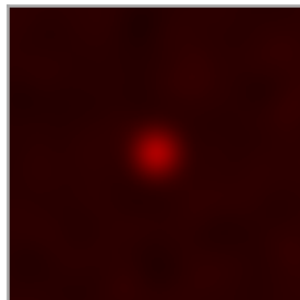
Gaussian2DKernel
