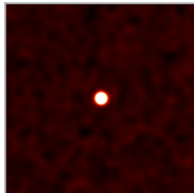
AiryDisk2DKernel
