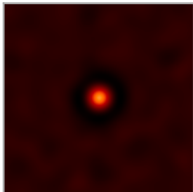
MexicanHat2DKernel
