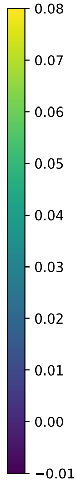
AiryDisk2DKernel
