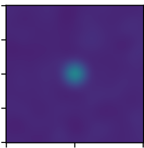
Gaussian2DKernel
