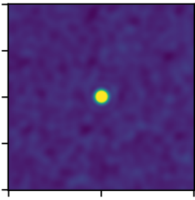
AiryDisk2DKernel
